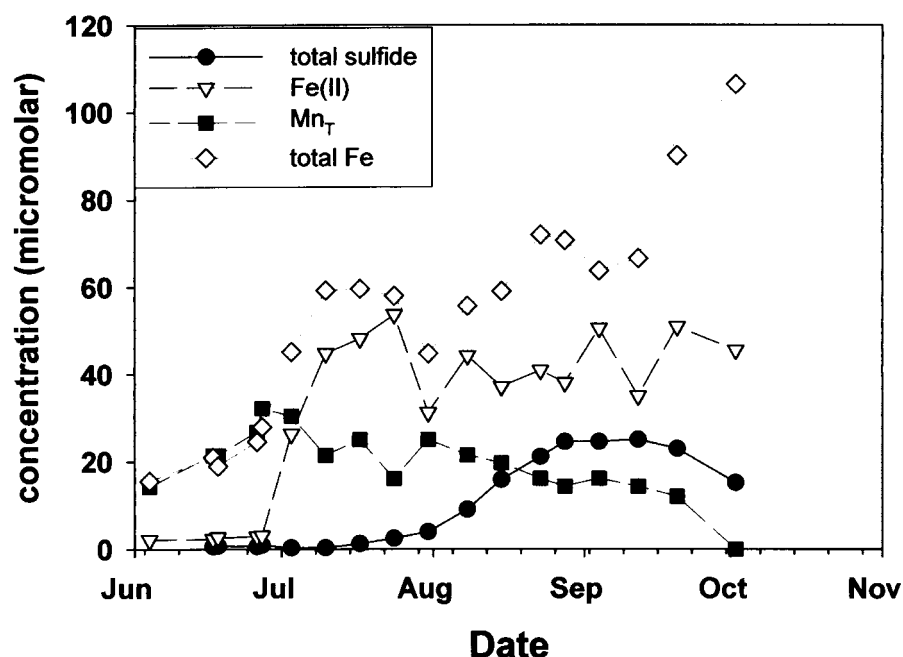
Figure 2. Seasonal data for Fe, S and Mn in the bottom waters of Lake Wallenpaupack at Wilsonville site 1.
