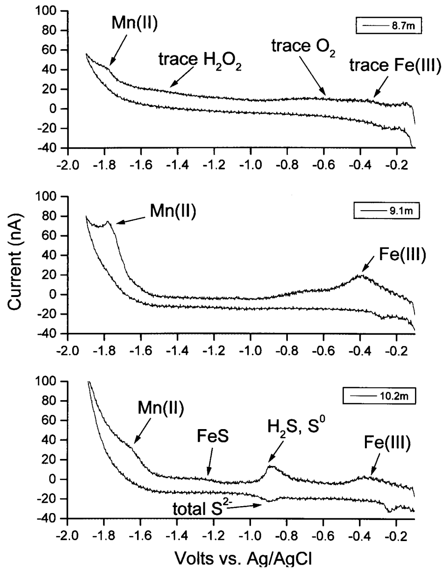
Figure 5. Cyclic voltammetric scans taken at the oxic-anoxic interface of Lake Wallenpaupak waters on Sept. 17, 2002 at site 2 at the dam forebay. Scan direction is from positive to negative then back to positive; scan rate is 1 V/sec. Mn 2+ , FeS, Fe(III)-organic complexes and S(0) (traces of H 2 S) are observed, but Fe 2+ is not detected.
