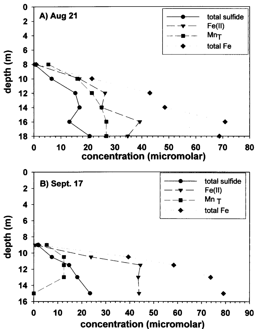
Figure 3. Representative profiles from analyses of discrete water samples taken from the Wilsonville site 1.
