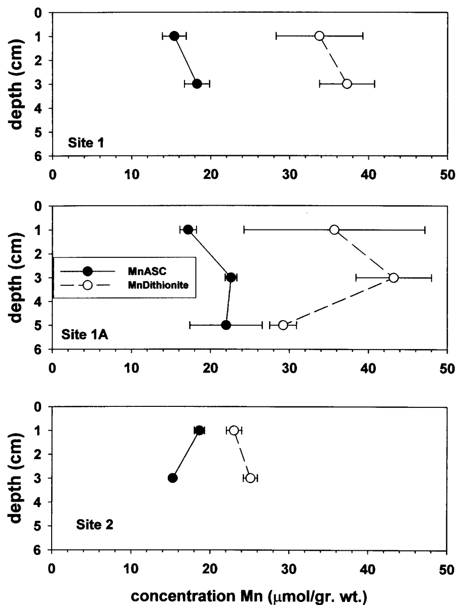
Figure 8. Solid phase Mn analyses versus depth. Depth is averaged since all cuts were 2 cm slices.
