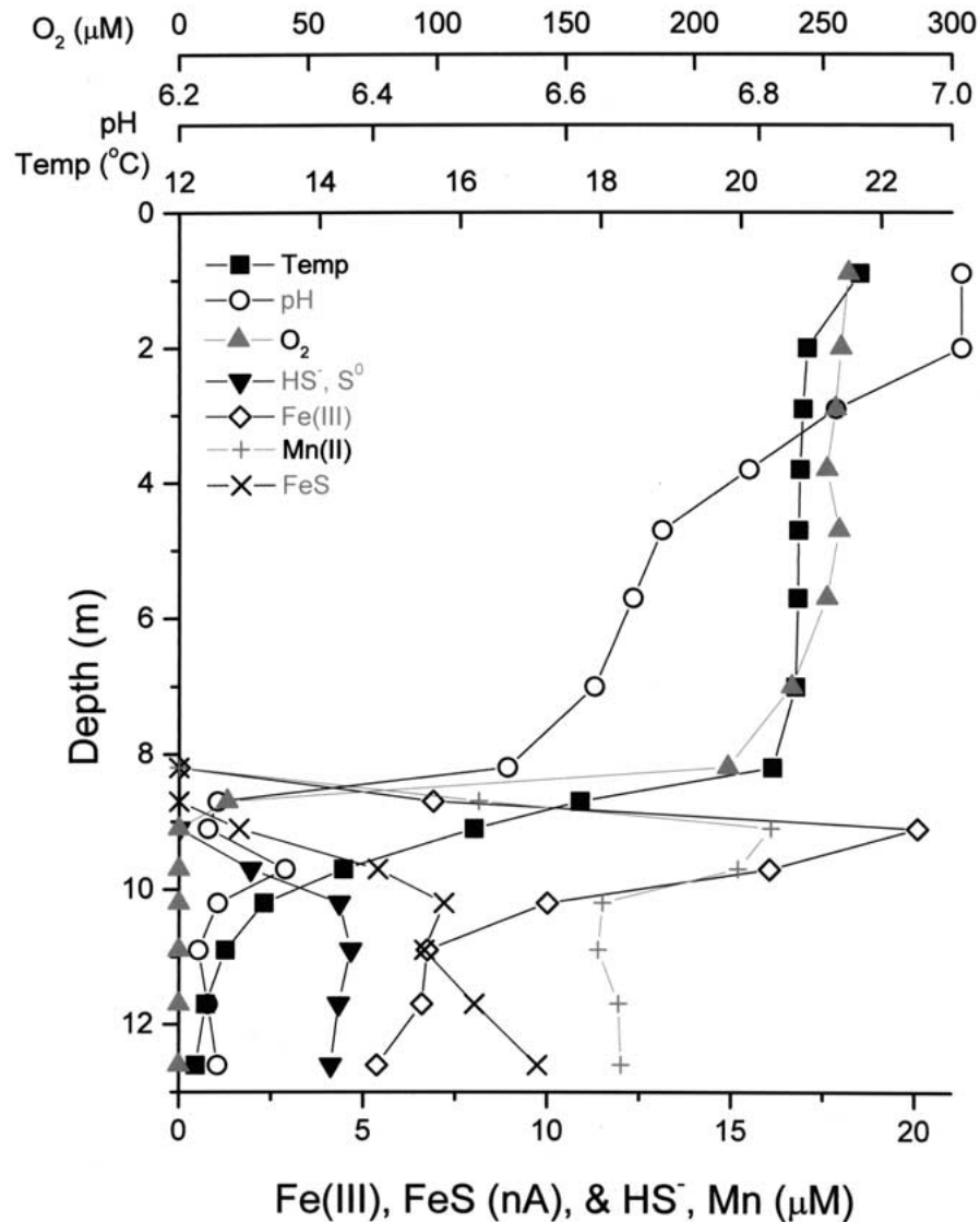
Figure 6. In situ profile for site 2 at the dam forebay on Sept. 17, 2002. O 2 and FeS overlap at the oxic/anoxic interface with a peak of Mn 2+ below the interface.
