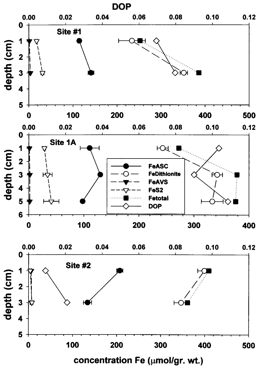
Figure 7. Solid phase Fe analyses and DOP versus depth. Depth is averaged since all cuts were 2 cm slices; i.e., 1 cm is the average from 0–2 cm.
