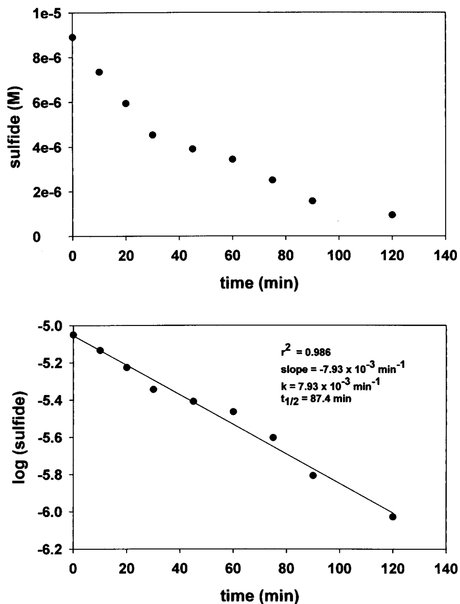
Figure 9. Kinetic data for waters sampled from the dam forebay on Sept. 19, 2002.
