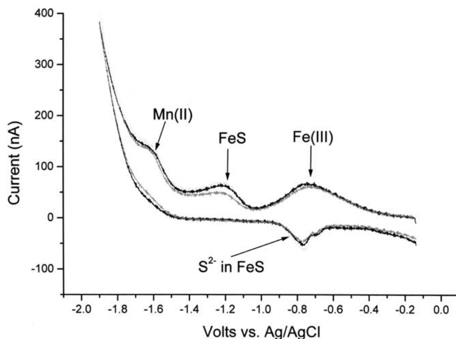
Figure 4. Cyclic voltammetric scans taken in Lake Wallenpaupak waters on Aug. 21, 2002 at site 3. Scan direction is from positive to negative then back to positive; scan rate is 1 V/sec. \text{Mn}^{2+} , FeS is observed, but free \text{H}_2\text{S} and \text{Fe}^{2+} are not detected.
