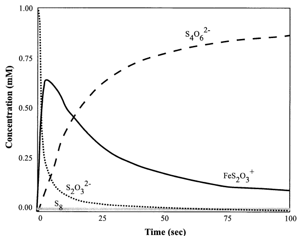
Fig. 11. Results of kinetic calculations for the fate of 1000 μM thiosulfate in a pH 1.5 solution containing 2 mM Fe 3+ . Note that negligible S 8 was formed as a result of disproportionation in this solution and that ~100% of the thiosulfate is converted to tetrathionate. Rate laws from Johnston and McAmish (1973) and Williamson and Rimstidt (1993) were used in this calculation.
