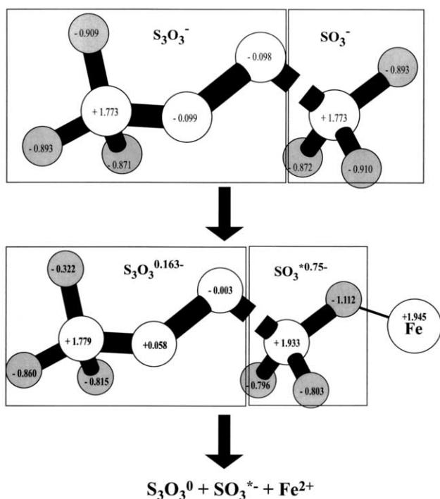
Fig. 12. gaussian98 calculations of tetrathionate and proposed transition state \text{FeS}_4\text{O}_6^+ , illustrating the degree of electron density shift as a result of \text{Fe}^{3+} -complexation and cleavage of a terminal S-S bond.
