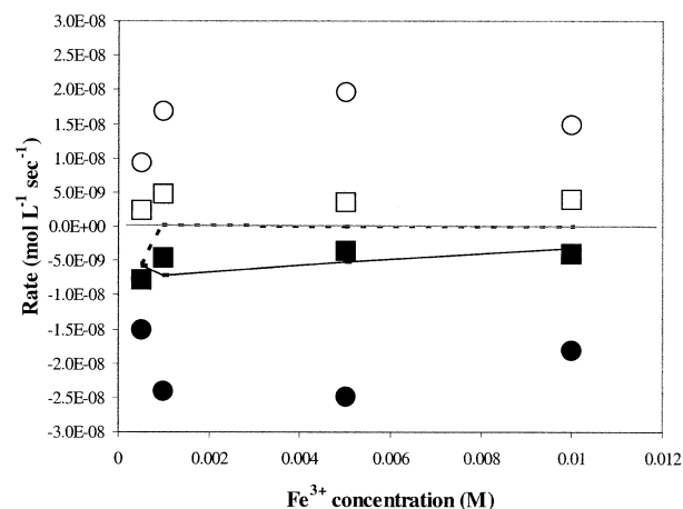
Fig. 7. Comparison of calculated rates for Series V experiments. Lines indicate the difference between rates calculated for directly measured S 4 O 6 2- (solid markers) and SO 4 2- (open markers). Round markers are rates calculated from initial rates while square markers are calculated from total rates. S 4 O 6 2- rates were normalized to 1 sulfur.
