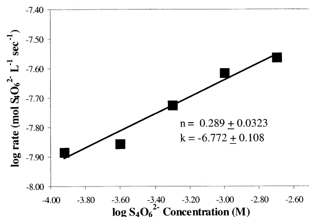
Fig. 6. - Log-log plot of initial rate of Series IV experiments vs. log variable [S_4O_6^{2-}]_{\text{initial}} , with 2 mM \text{Fe}^{3+} , pH 1.5, at 70°C (rate data available in Table 3 and Table A1).
