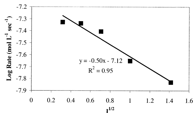
Fig. 8. Dependence of tetrathionate decomposition rates on ionic strength (I) in Series VI experiments. After the Bronsted equation, relating ionic strength to kinetics, the negative slope indicates reaction between oppositely charged species where greater ionic strength effectively shields the range of electrostatic interaction.
