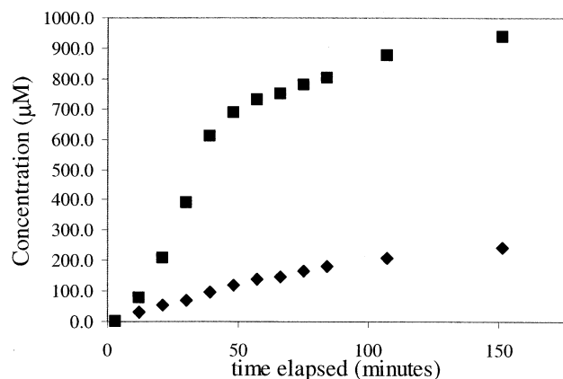
Fig. 10. Diagram of a trithionate oxidation experiment with 500 μM S 3 O 6 2- at 35°C in a pH 1.5 solution with 2 mM Fe 3+ . The squares represent SO 4 2- and the diamonds represent Fe 2+ measured in the course of the experiment.
