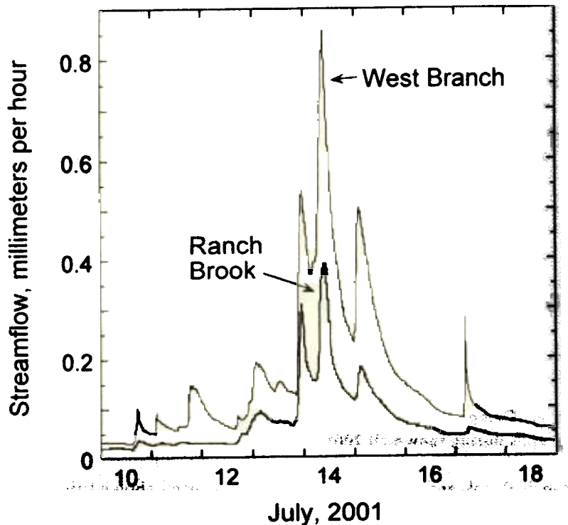
Figure 5. Comparison of West Branch and Ranch Brook streamflow hydrographs during a series of rainstorms in July, 2001.
