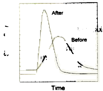
Figure 2. Theoretical shift in storm hydrograph to earlier and higher peak flows as a result of land disturbance and/or development.
